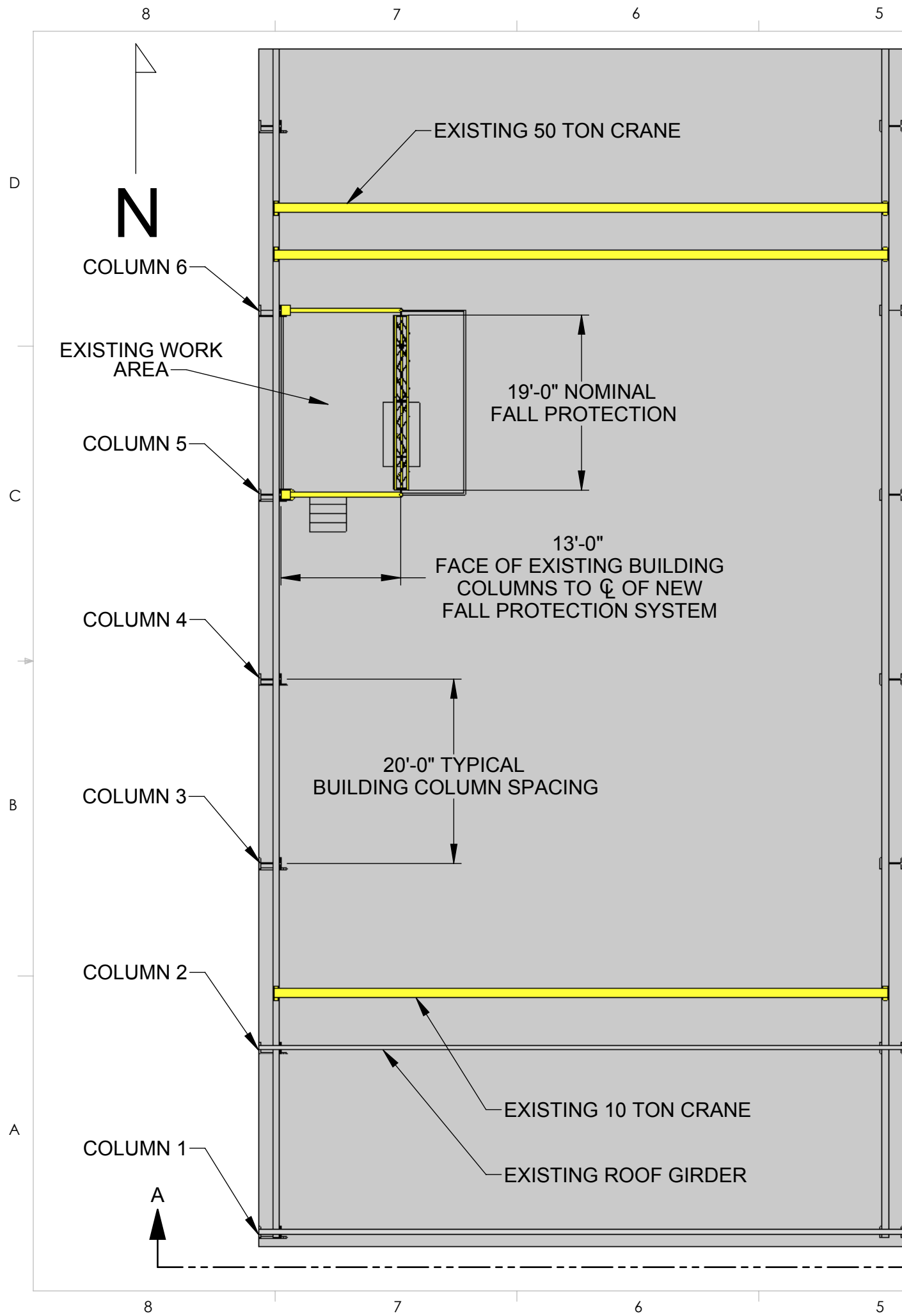
PLAN VIEW
